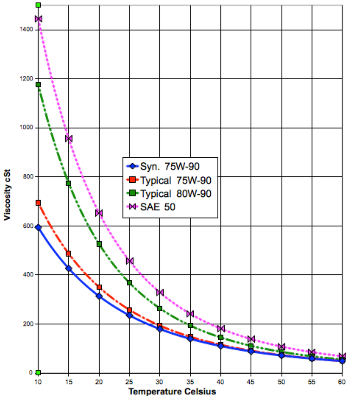
Viscosity Curve
