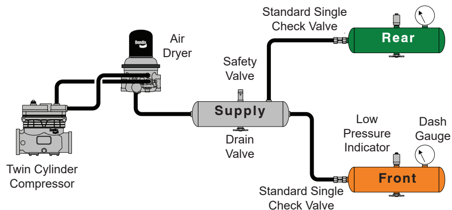
Conventional Supply System & Bendix® AD-9si® Air Dryer
