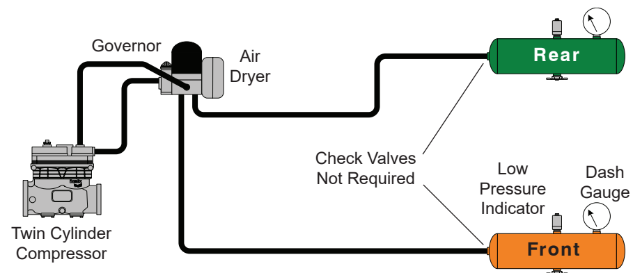
Two Reservoir Supply System & Bendix® AD-IS® Air Dryer
