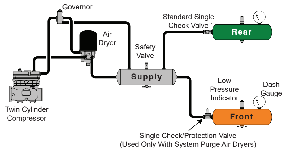
Conventional Supply System & System Purge Air Dryer
