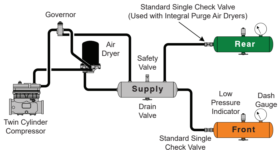
Conventional Supply System & Integral Purge Air Dryer
